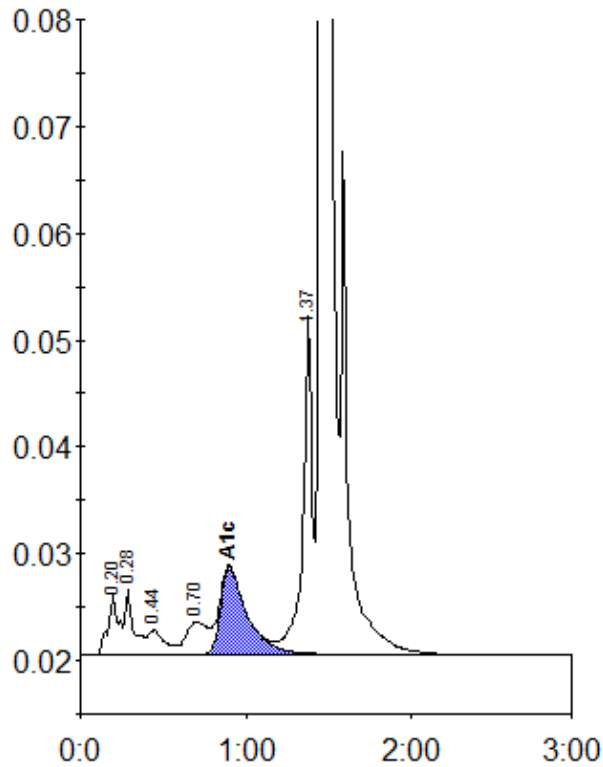
Peak table - ID: 10316424
